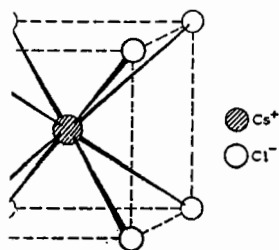
3.6 Caesium chloride structure. (Reproduced by permission of Wells, A.F., Inorganic Chemistry , Oxford University Press,
