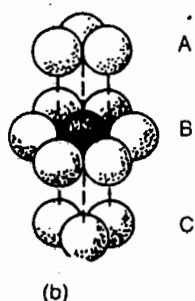
Figure 2.5 Arrangement of 12 neighbours in hexagonal close-packed (a) and cubic close-packed (b) structures. (Note that the top and bottom layers are the same, but the bottom layer in the cubic close-packed structure is rotated 60° relative to the hexagonal close-packed.)
