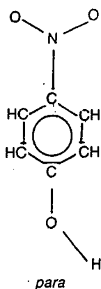
3.5 Structures of ortho , d para nitrophenol.
