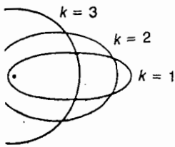
5 Bohr-Sommerfeld orbits for n = 3 .
